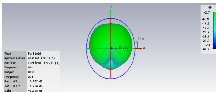
Fig-13, 3D Far field radiation pattern of antenna at 2.1 Ghz
