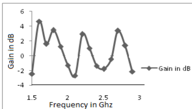
Fig-7, variation of gain over the frequency range
