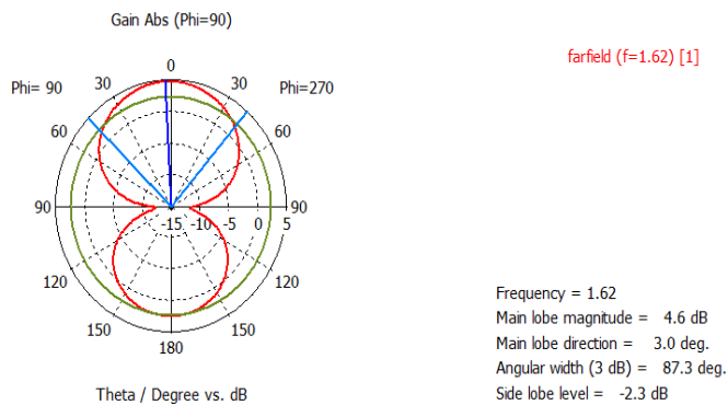
Fig-10, polar plot of monopole antenna at 1.62 Ghz
