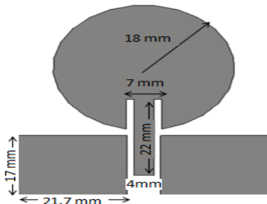
Fig-2, geometry of monopole antenna with EBG structure
