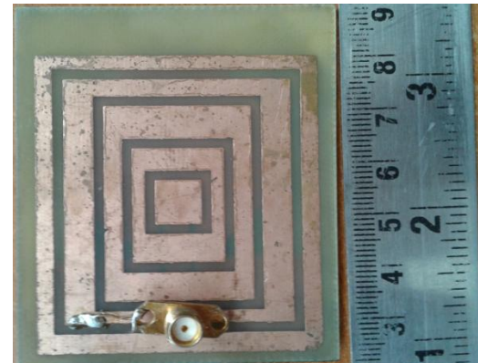
Fig-5, Fabricated view of ground with rectangular slots
