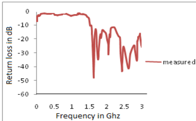
Fig-6, Measured return loss of fabricated monopole antenna
