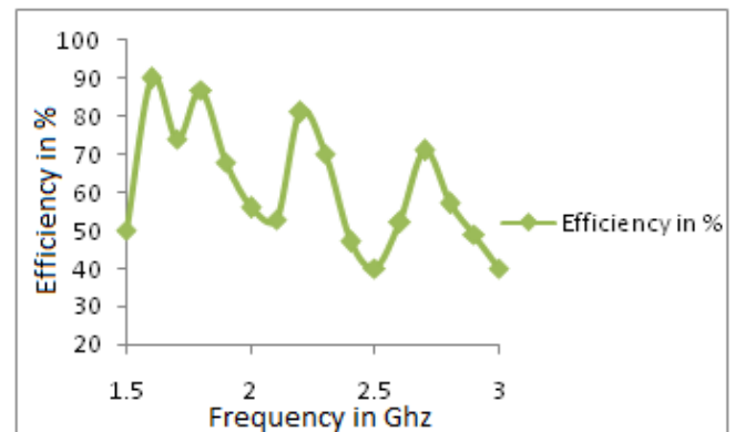
Fig-9, Efficiency of monopole antenna
