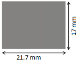
Fig-1, unit cell of EBG structure
