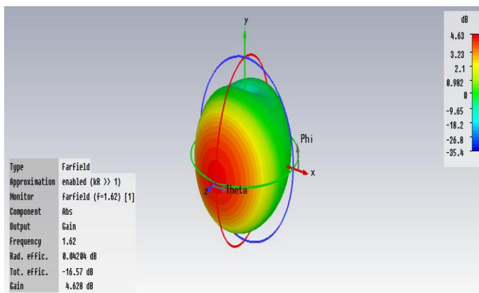
Fig-12, 3D Far field Radiation pattern of antenna at 1.62 Ghz
