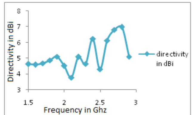
Fig-8, variation of Directivity over the frequency band
