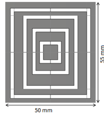
Figure-3, geometry of ground plane with rectangular slots
