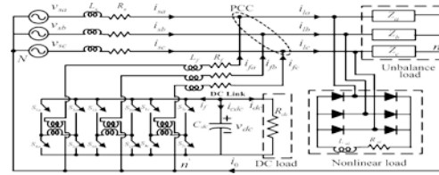
Fig. 1. Three-phase, four-wire compensated system using the H-bridge VSI topology-based DSTATCOM.
