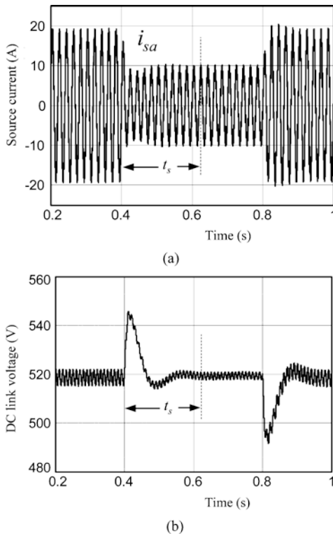
Fig. 5. Transient response of the conventional controller. (a) Compensated source current in phase \alpha . (b) DC-link voltage.
