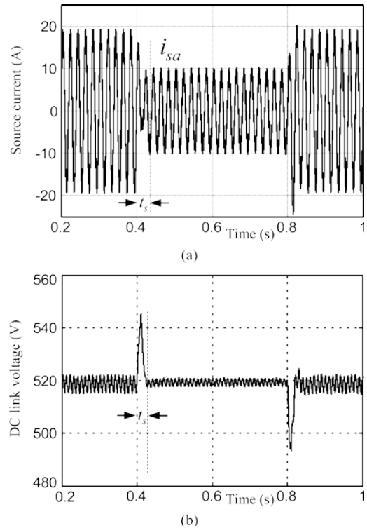
Fig. 6. Transient response of the fast-acting controller. (a) Compensated source current in phase \alpha . (b) DC-link voltage.
