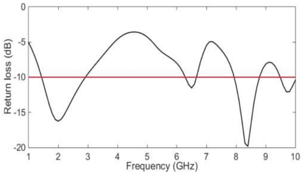
Figure 6. Return loss plot of proposed antenna with H L =2.0mm
